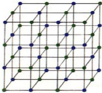
Crystalline three-dimensional-lattice-structure
